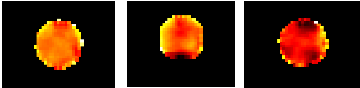
Baseline (a) PV: 0.1322 \mu\text{m} Optic 13446 (b) PV: 0.1347 \mu\text{m} RMS: 0.0088 \mu\text{m} Optic 13447 (c) PV: 0.1051 \mu\text{m} RMS: 0.0059 \mu\text{m}
